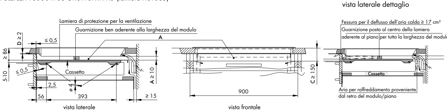
Piano cottura: FULLFLEX V6000 I705 CTI6T75FKTFHD (lamiera H61085/H61083)
