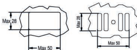
FORO TPR / OVERFLOW HOLES
